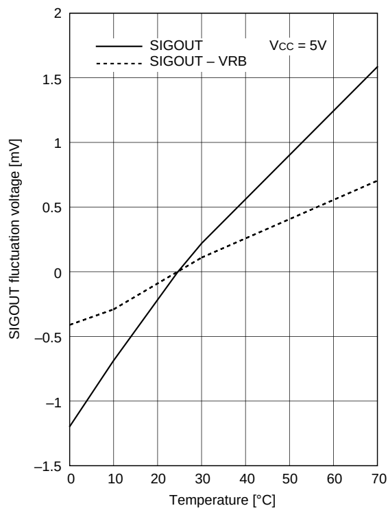
Clamp voltage temperature characteristics fluctuation
