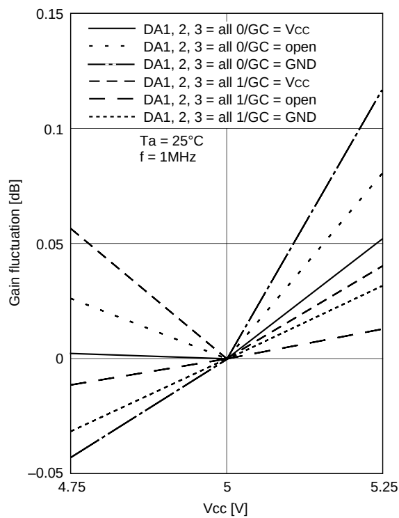
Total gain supply voltage fluctuation
